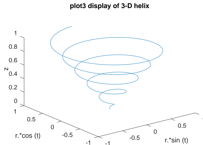
Figure 15.6: Three-dimensional spiral.
