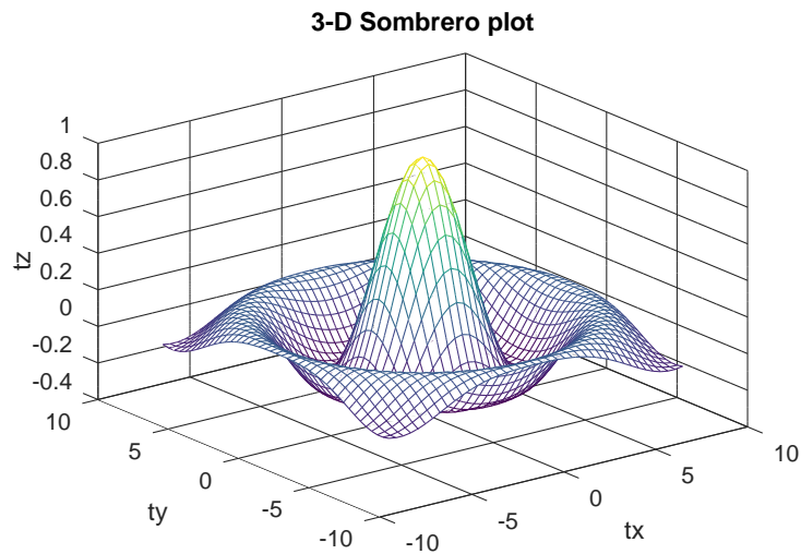
Figure 15.5: Mesh plot.
