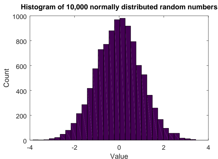
Figure 15.2: Histogram.
