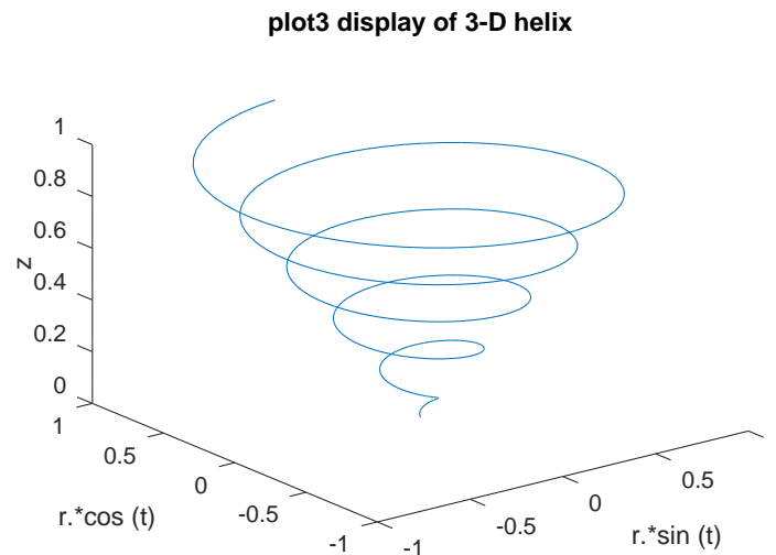
Figure 15.6: Three-dimensional spiral.
