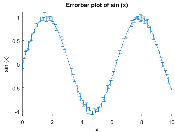
Figure 15.3: Errorbar plot.
